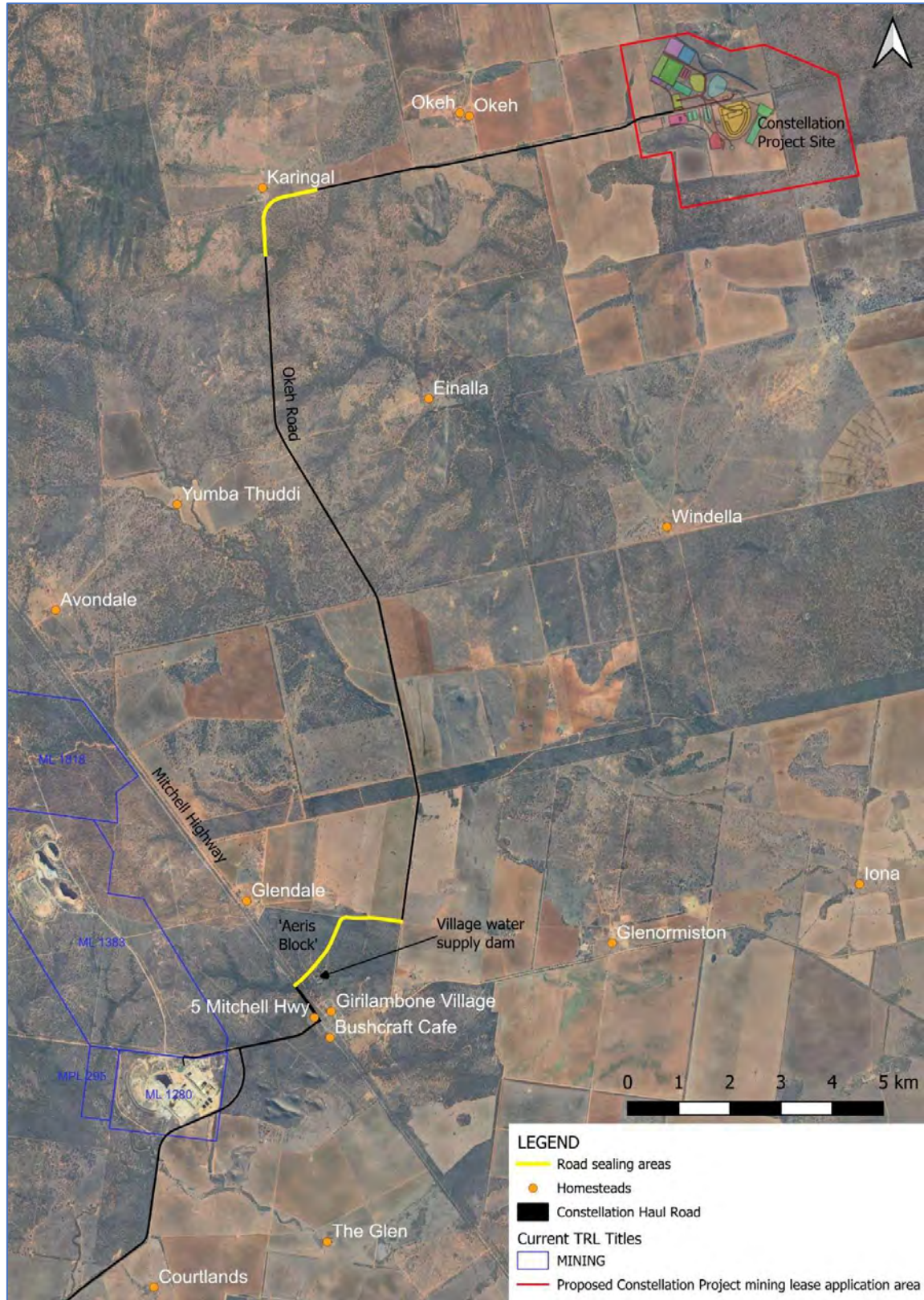
Figure 10 Constellation Project minimum road seal areas
